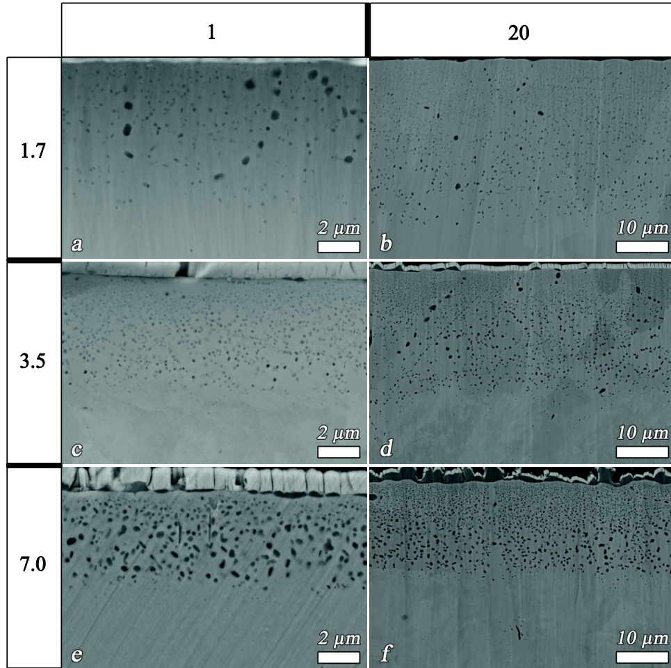
Figure 2 Backscattered electron images of cross sections of Mn-steel alloys oxidized for 1 and 20 h at 950 °C in N 2 plus 5 vol.% H 2 with a dew point of 10 °C. The images in the first and second columns correspond with 1 and 20 h oxidation, respectively. The images in the first, second and third rows correspond with the Mn fraction in wt%, respectively. The bright layer on top is a metallic layer applied for sample preparation.
