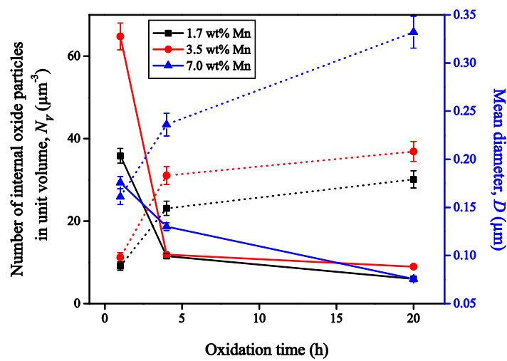
Figure 1 Number of internal oxide particles per unit volume versus oxidation time for three Mn-steel alloys oxidized at 950 °C in \text{N}_2 plus 5 vol.% \text{H}_2 with a dew point of 10 °C. The mean diameters of internal oxide precipitates are shown as dashed lines.
