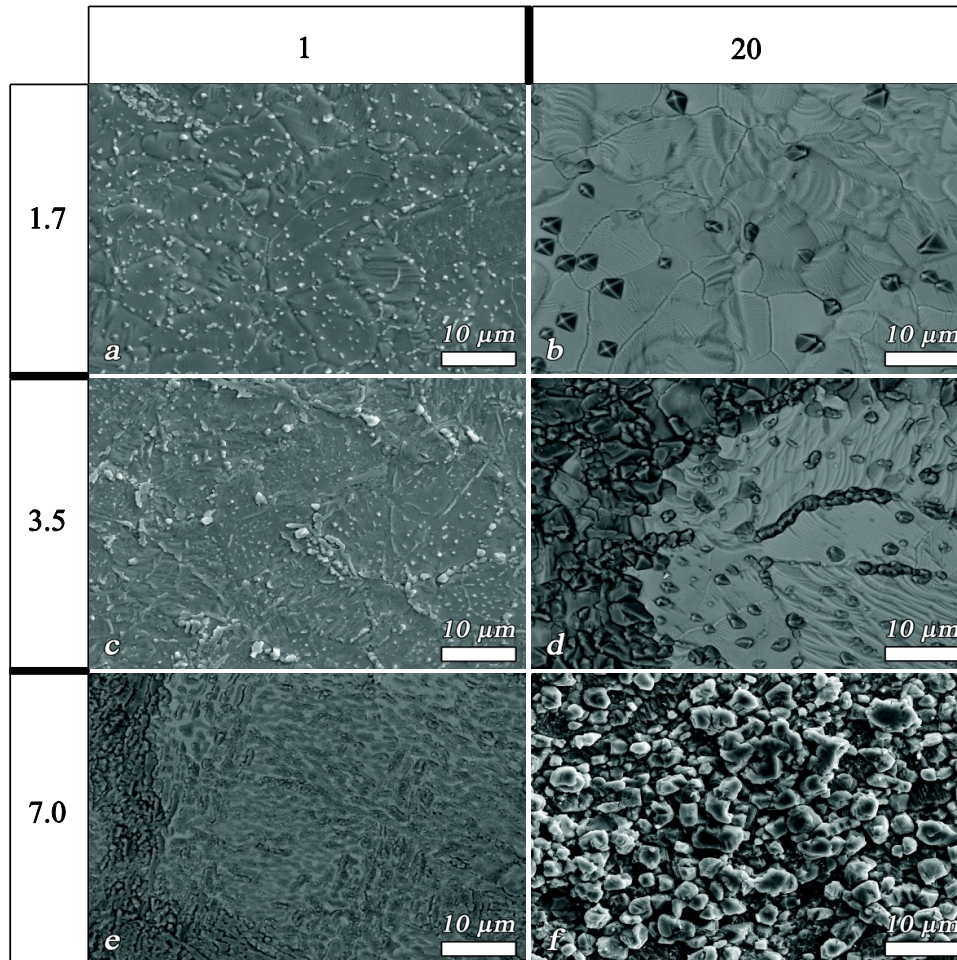
Figure 5 Secondary and backscattered electron images of surface of the Mn-steel alloys oxidized for 1 and 20 h at 950 °C in N 2 plus 5 vol.% H 2 with a dew point of 10 °C. The images in the first and second columns correspond with 1 and 20 h oxidation, respectively. The images in the first, seconds and third rows correspond with the Mn fraction in wt%, respectively.
