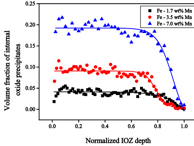
Figure 3 Volume fraction of internal oxide precipitates versus the normalized depth of internal oxidation zone in Mn-steel alloys oxidized for 20 hours at 950 °C in N 2 plus 5 vol.% H 2 with a dew point of 10 °C.
