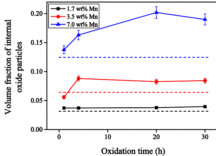
Figure 4 Volume fraction of internal oxide particles versus oxidation time of Mn-steel alloys oxidized at 950 °C in N 2 plus 5 vol.% H 2 with a dew point of 10 °C. The dotted lines correspond to the volume fraction of internal oxides if the total amount of Mn in the internal oxidation zone was transformed into MnO (i.e. no enrichment and deviating stoichiometry).
