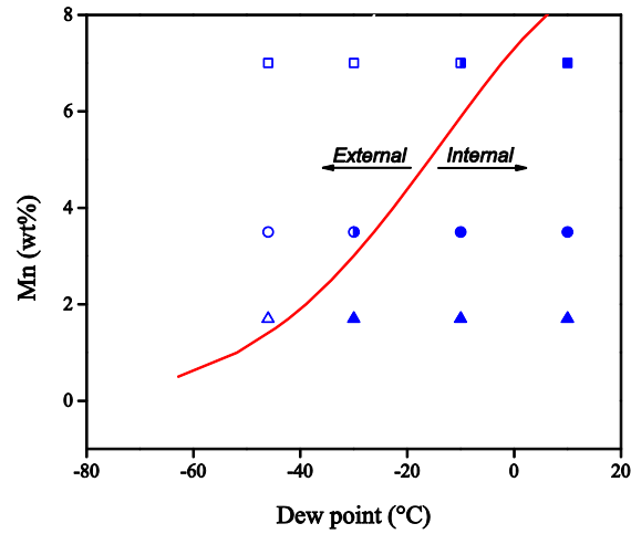
Figure 6 Oxidation domains for binary Fe-Mn alloys at 950 °C as a function of dew point in a mixture of N 2 plus 5 vol.% H 2 using the general criterion, cf. Eq. (7). The line depicting the transition from internal to external oxidation is determined using 0.2 as the critical volume fraction of internal oxides and the diffusion coefficients of oxygen and manganese as obtained from the observed internal oxidation kinetics and Mn concentration depth profiles, respectively. For the molar volume of the oxide the value of stoichiometric MnO [14] was adopted. The filled, unfilled and half-filled symbols represents: internal, external and simultaneous internal and external oxidation modes, respectively.
