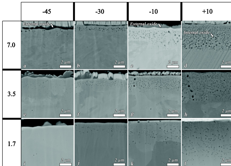
Figure 7 Backscattered electron images of cross sections of Mn-steel alloys oxidized for 1 (at dew points of 10, -10 and -30 °C) and 4 h (at dew point of -45 °C) at 950 °C in N 2 plus 5 vol.% H 2 with various dew points, see Figure 6 for external versus internal oxidation. The images in the first till the fourth columns correspond with the dew points in °C. The images in the first, seconds and third rows correspond with the Mn fraction in wt%, respectively. The bright layer on top is a metallic layer applied for sample preparation.
